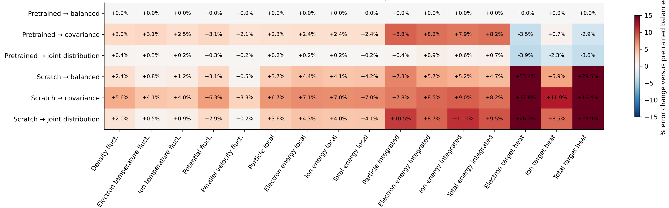
Same validation volumes · where each loss helps or hurts (blue = lower error)
